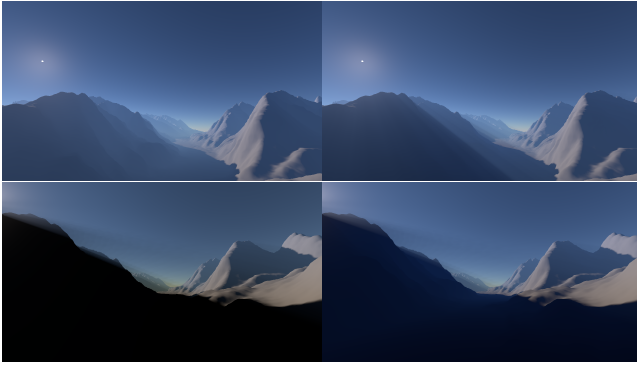
Figure 3: Top: a scene with sun, sky and aerial perspective without (left) and with (right) volumetric shadows. Bottom: images present a ground view when multiple scattering is evaluated (right) or not (left). Note: global illumination on the terrain is disabled to make observations more visible.
