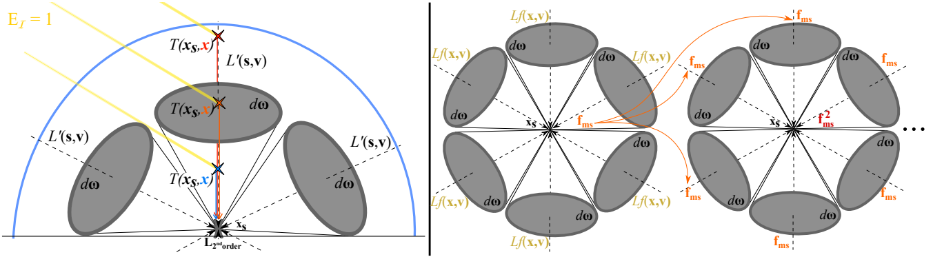
Figure 8: Sketch presenting on the left how L_2^{nd\_order} is computed from single scattering L' and, on the right, how F_{ms} approximates multiple scattering bounces using a normalized transfer function f_{ms} , corresponding to Equation 7, and assuming a sample point neighborhood receive the same amount of energy as the sample point itself, corresponding to Equation 9.
