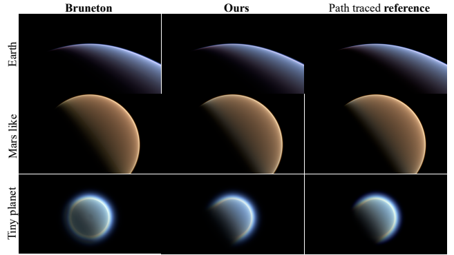
Figure 10: Space view rendering of different planets: Earth, Mars like and a fictional tiny planet with a thick and dense atmosphere.
